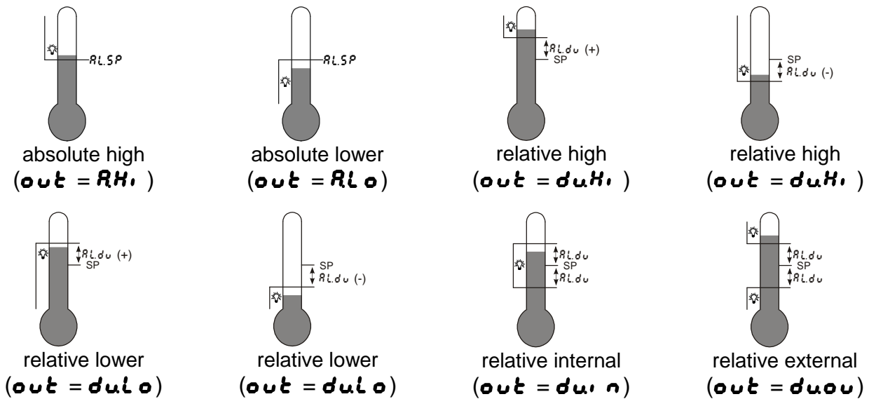
Fig.14. Types of alarms
