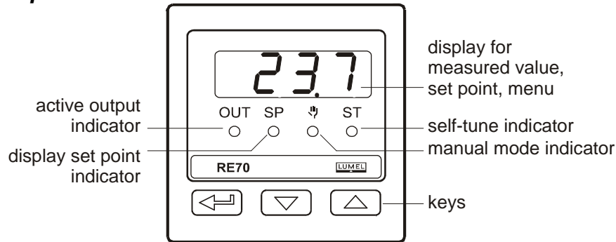
Fig. 8. Overview of the controller's front panel.
