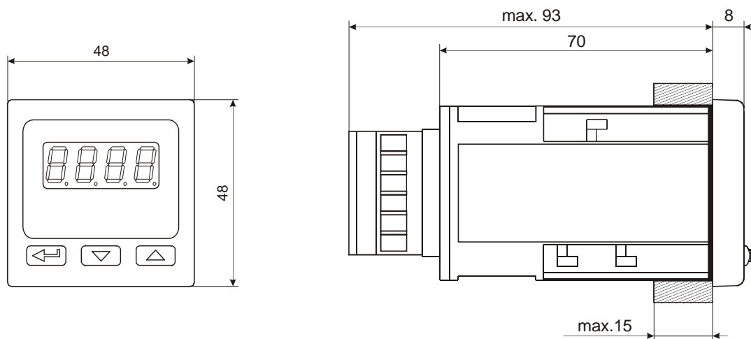
Fig. 2. Controller dimensions.
