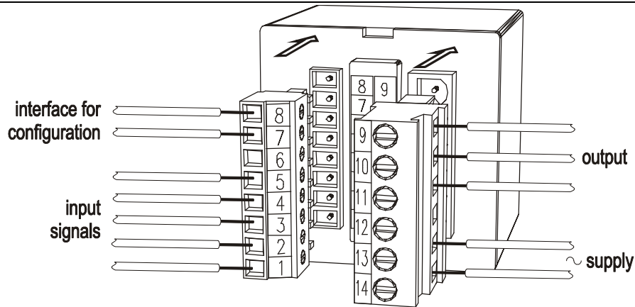
Fig. 3. View of the controller's connection strips.
