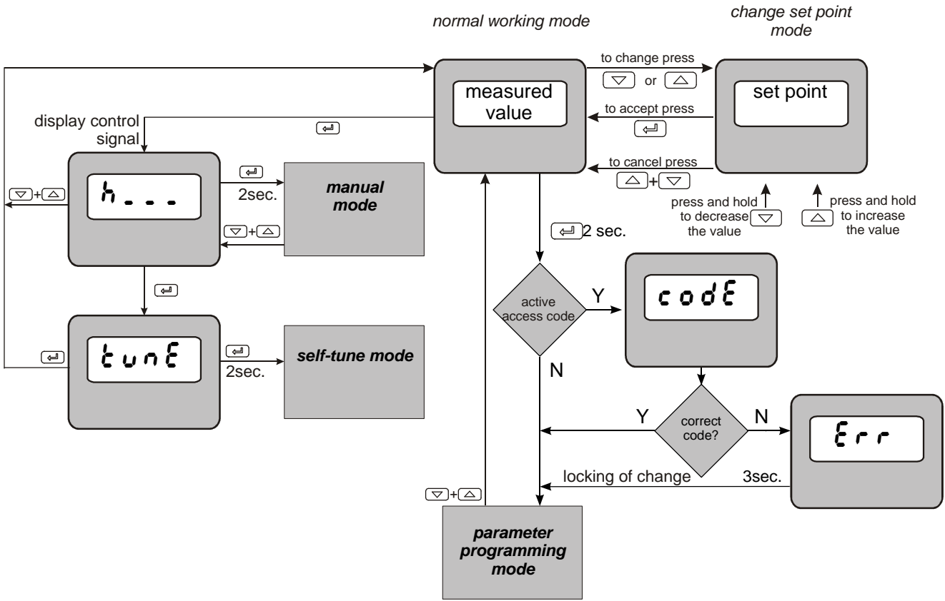
Fig. 10. Menu of controller service
