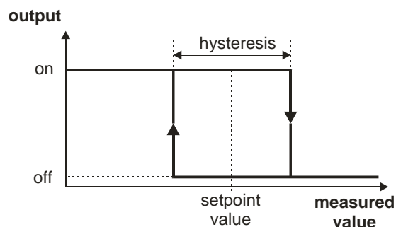
Fig. 13. Operation way of the heating type output for the ON-OFF control.
