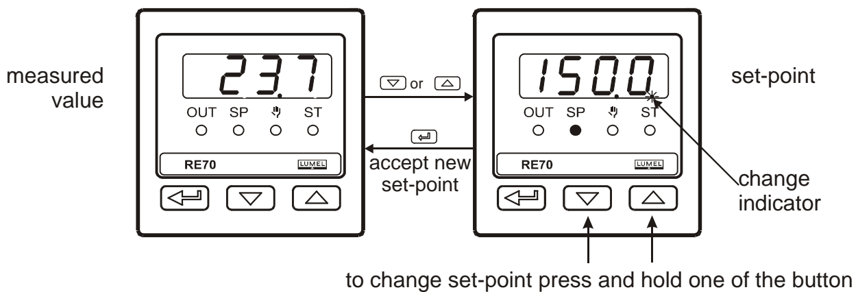
Fig. 9. Change value of the set point.
