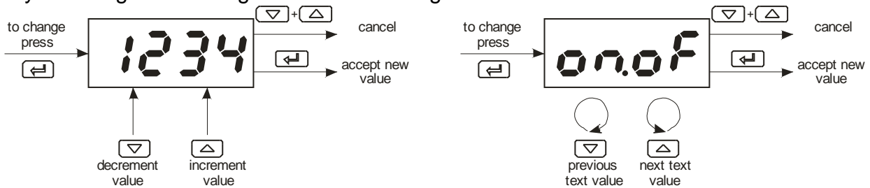
Fig. 12. Setting change of number and text parameters.
