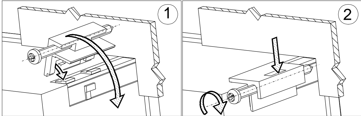
Fig. 1. Controller installation.
